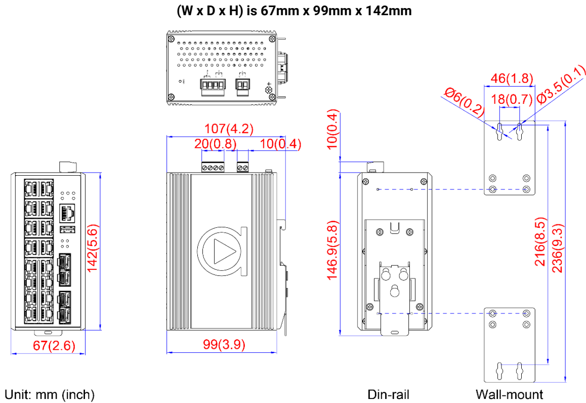
Figure 2.1 - Physical Dimensions
